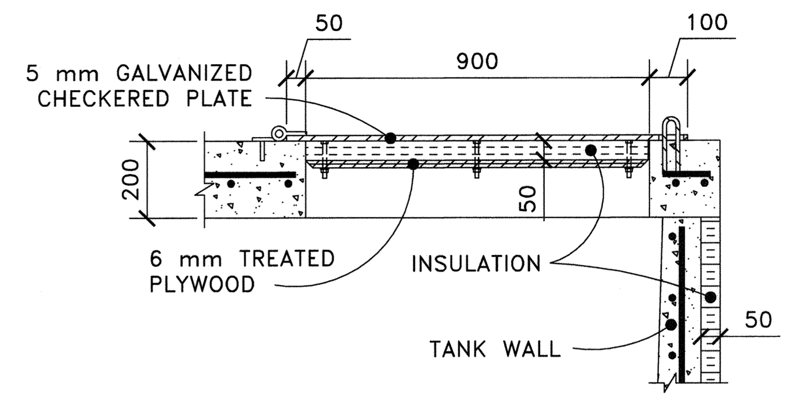
1 SECTION, THROUGH ACCESS HATCH N.T.S.
