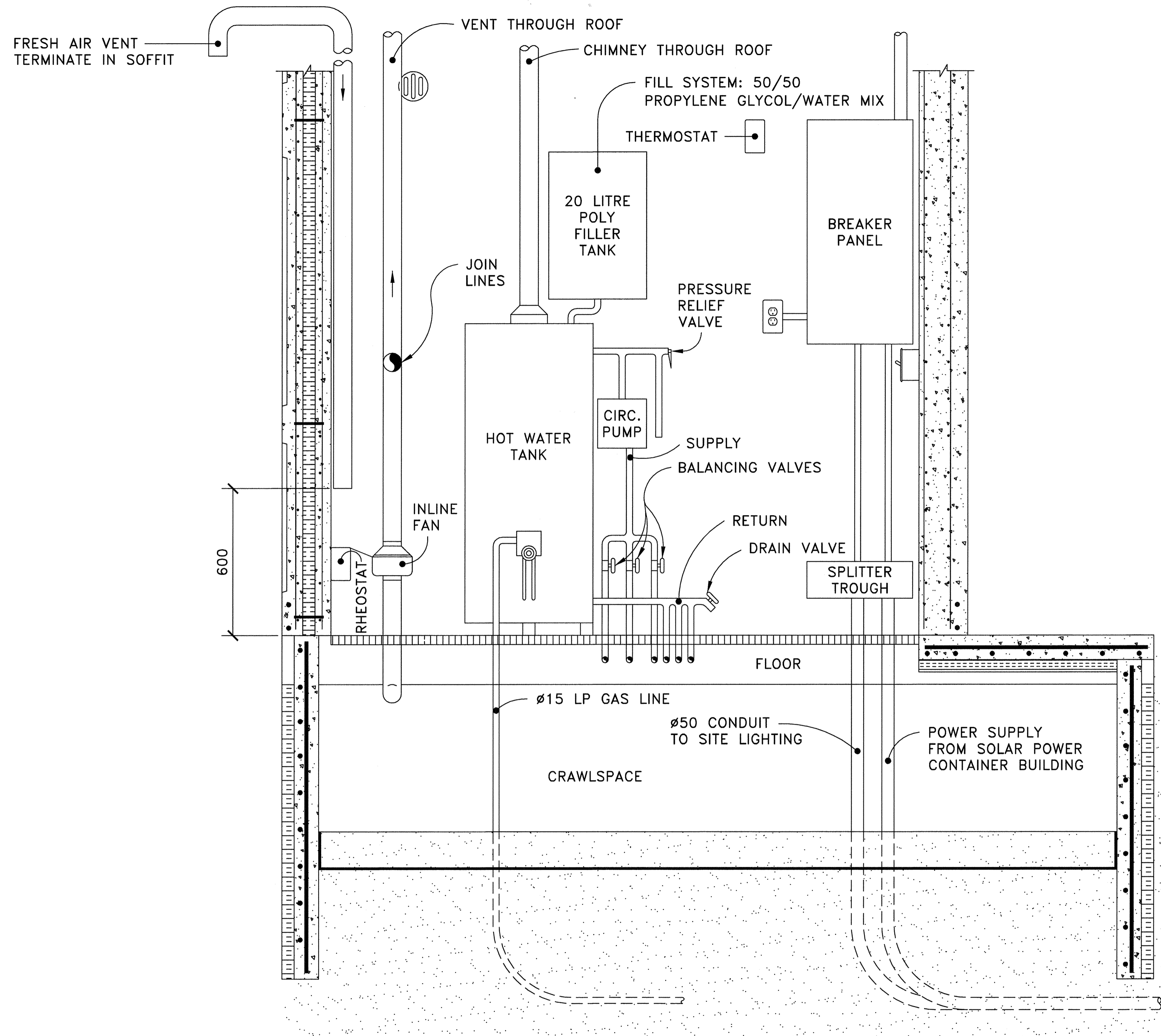
2 SECTION THROUGH MECHANICAL ROOM OF SOLAR POWER TOILET CB6-4.6M16 N.T.S.
