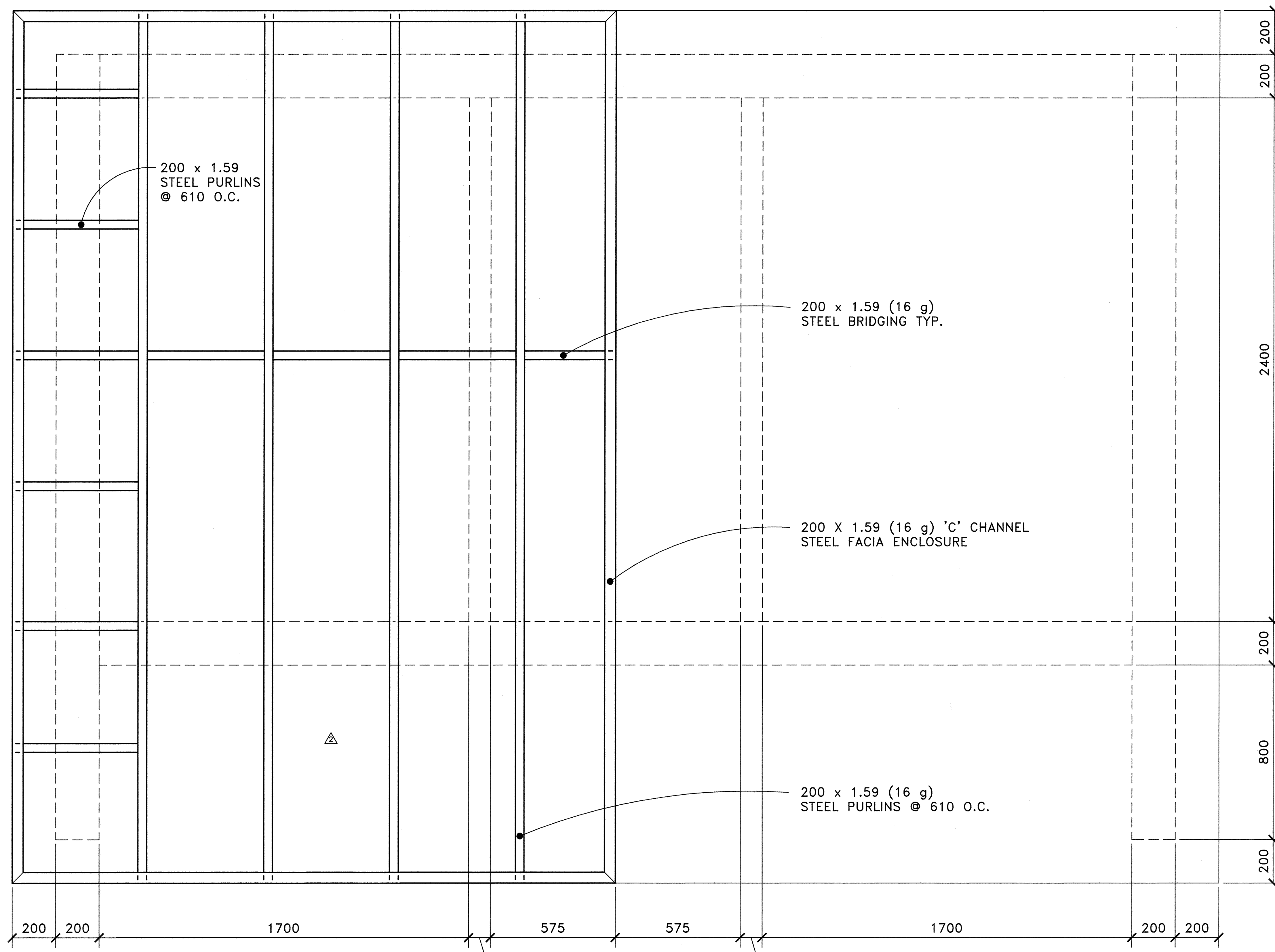
ROOF FRAMING PLAN N.T.S.
