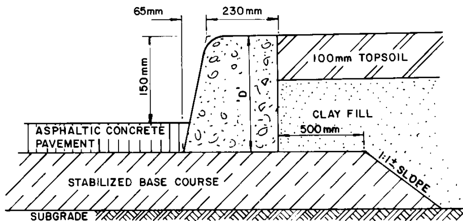
DETAIL OF CURB
