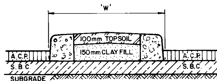
CROSS-SECTION AT TURNING LANE
