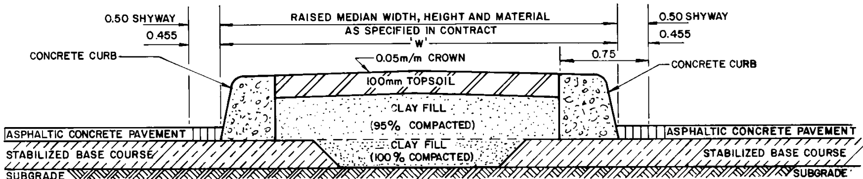
CROSS - SECTION
