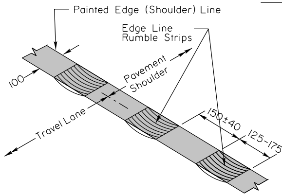
GAP EDGE LINE RUMBLE STRIP INSTALLATION
