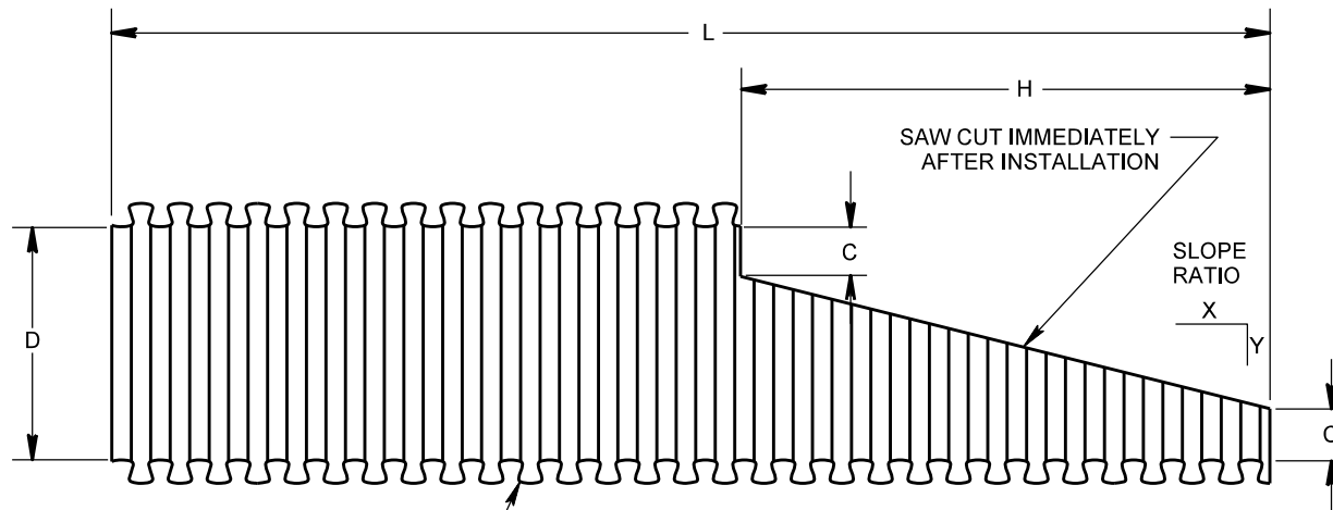
EXAMPLE OF CORRUGATED POLYETHYLENE PIPE (C.P.P.)
