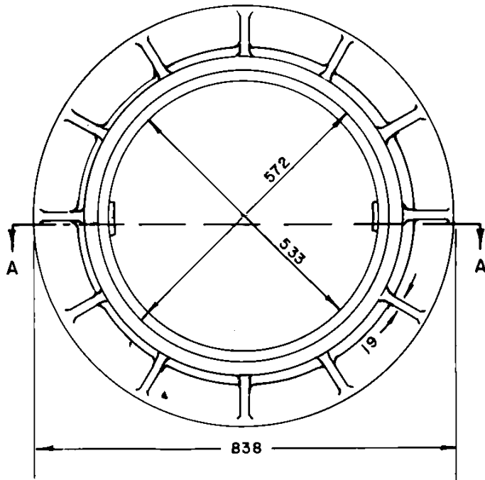
FRAME-PLAN VIEW
