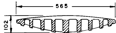
SECTION B - B
