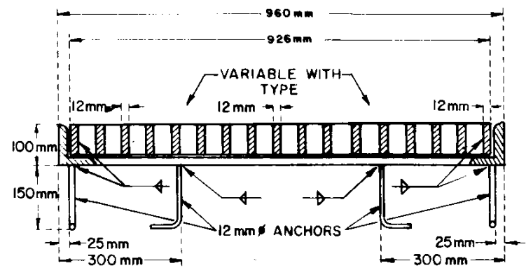
LONGITUDINAL SECTION THROUGH FRAME AND GRATE
