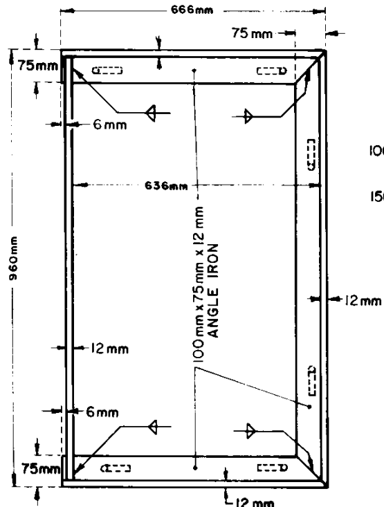
WELDED GRATE FRAME
