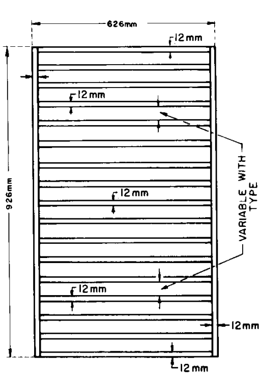
WELDED GRATE
