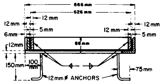
CROSS SECTION THROUGH FRAME AND GRATE
