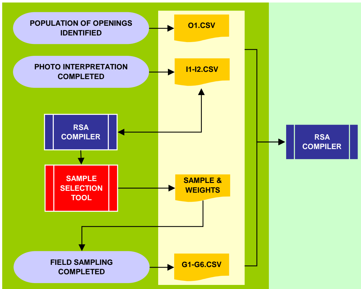
Figure 7. General data flow for the Aerial Stratification System.
