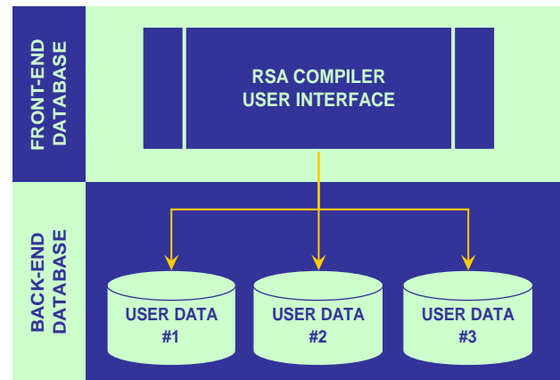
Figure 4. RSA Compiler split database design.
