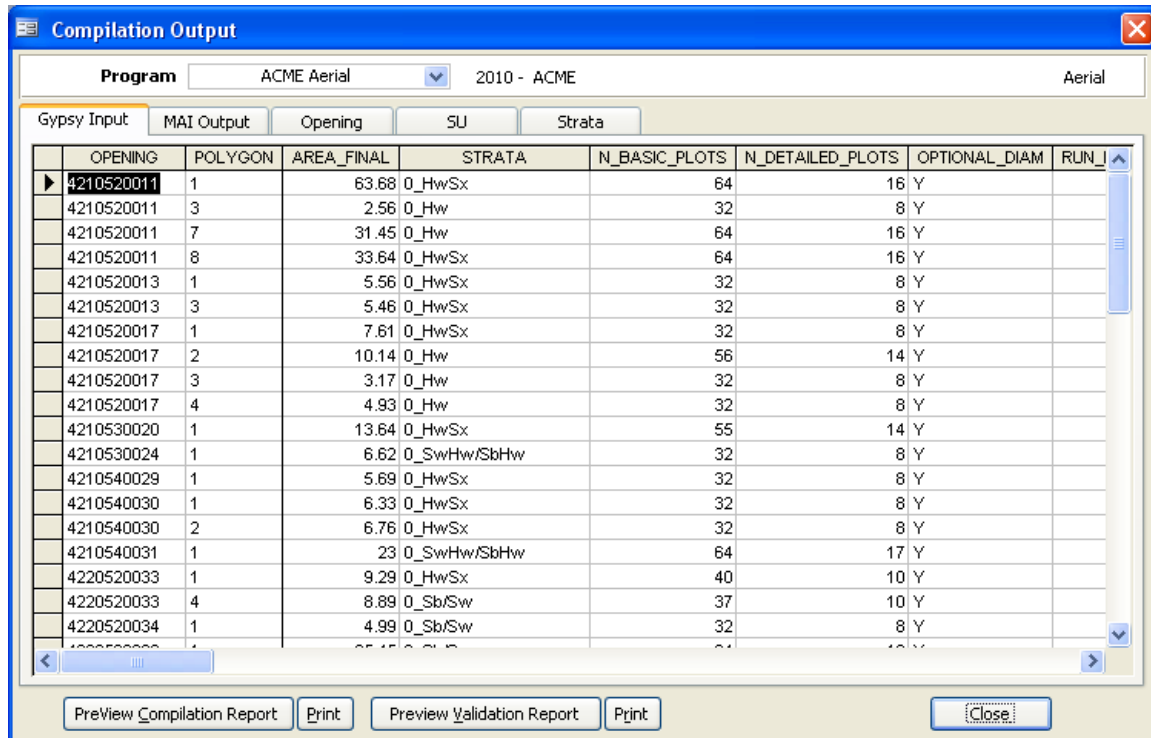
Figure 17. Compilation output.
