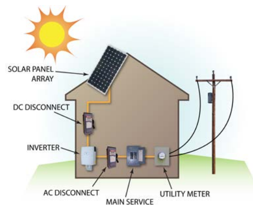
Figure 3 – PV Modules Net Metered Arrangement - Photo credit – Google Images
