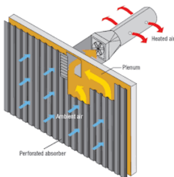
Figure 10 – Solar wall schematic – Photo credit – Google
