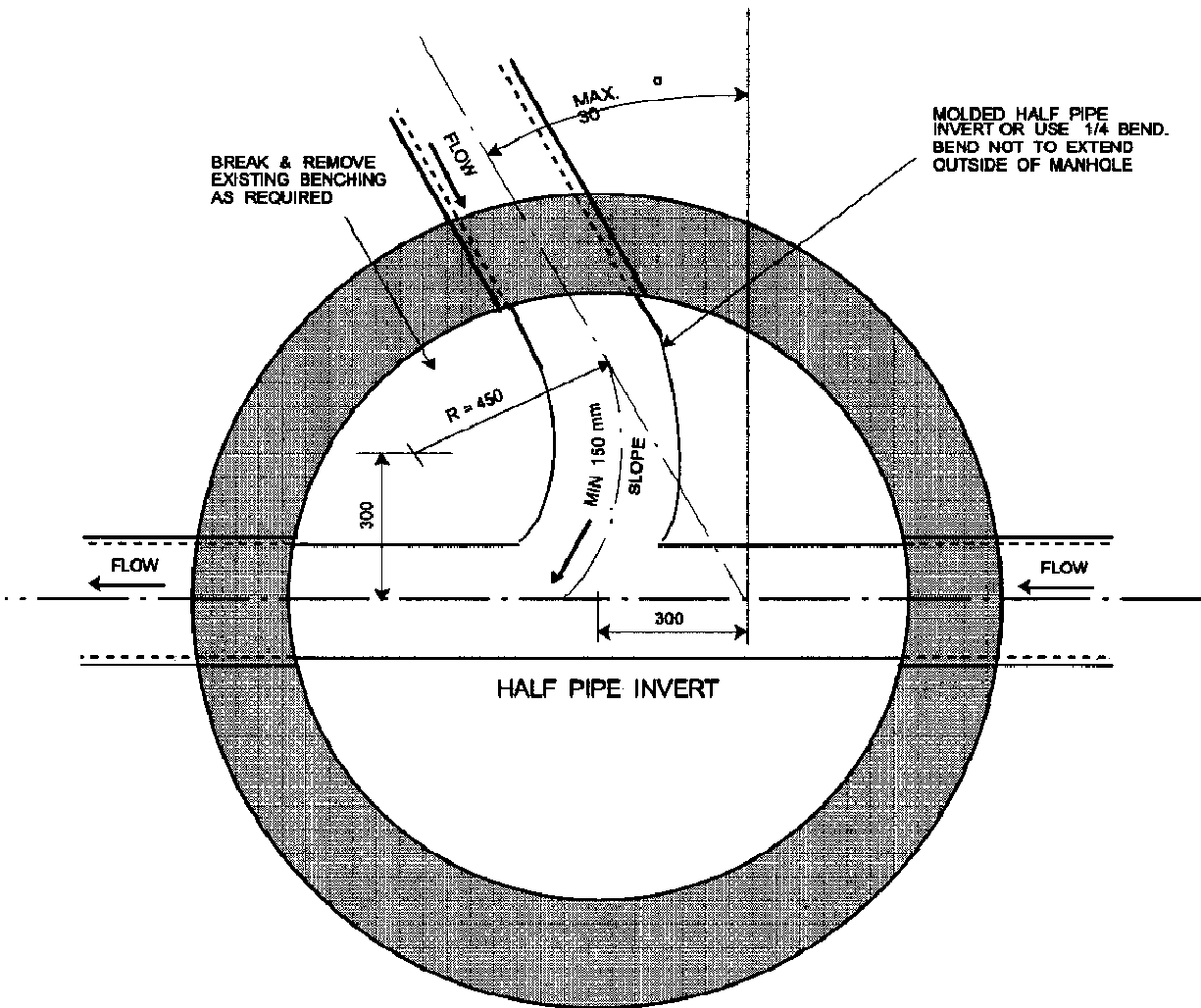
STANDARD 1200 mm MANHOLE
