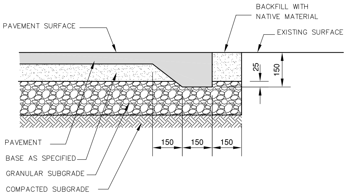
SECTION DETAIL
