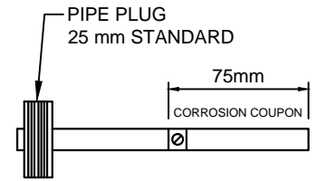
316 Stainless Steel Corrosion Coupon Holder
