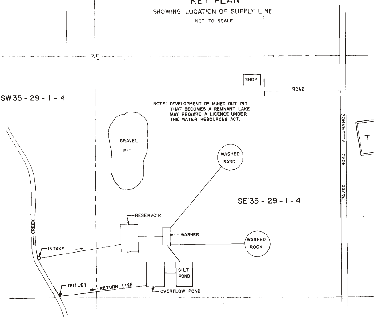
GENERAL PLAN SHOWING INTAKE AT CREEK & OUTLET FROM RETURN LINE NOT TO SCALE
