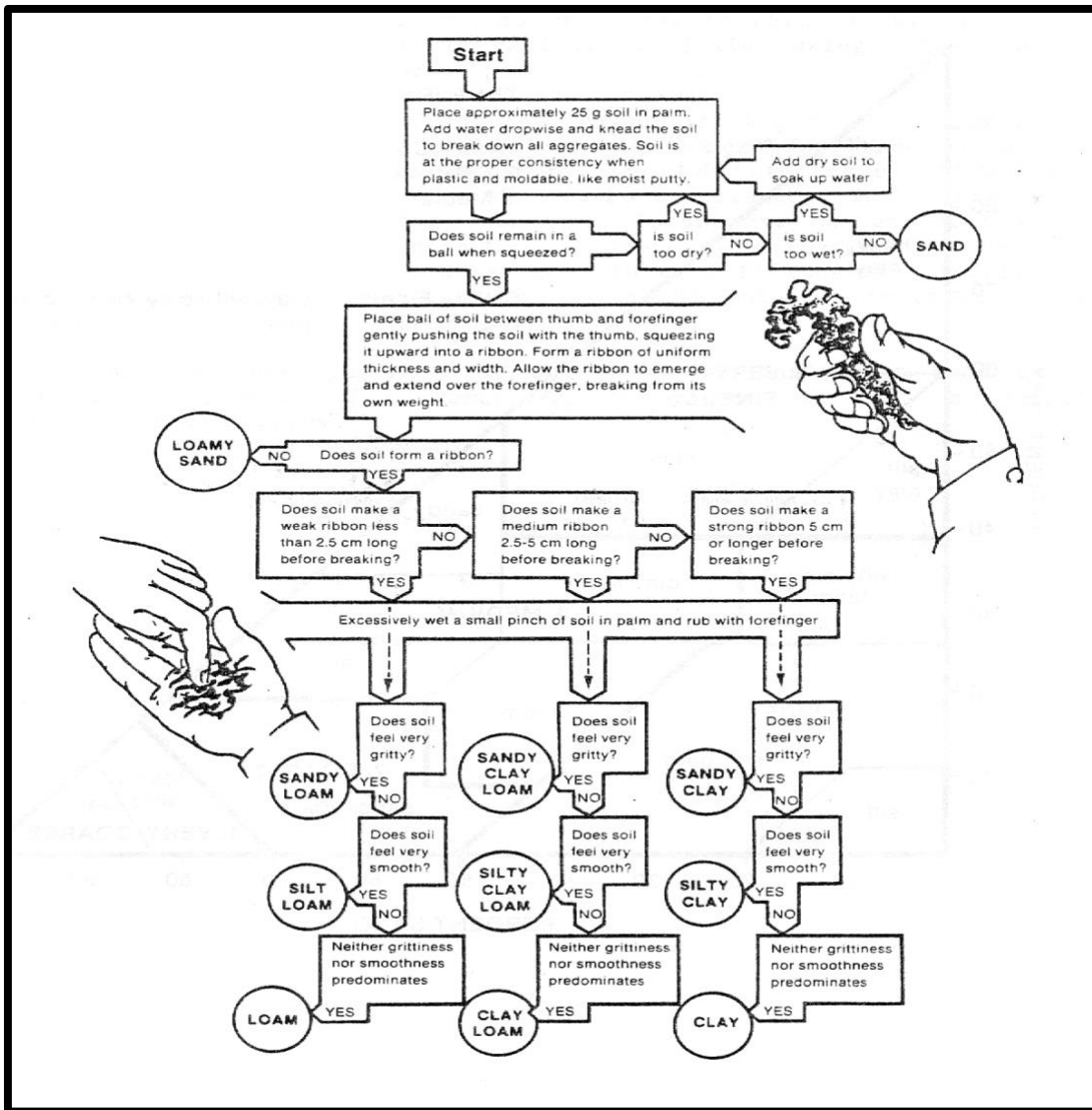
Figure 6. Determining soil texture by hand.
