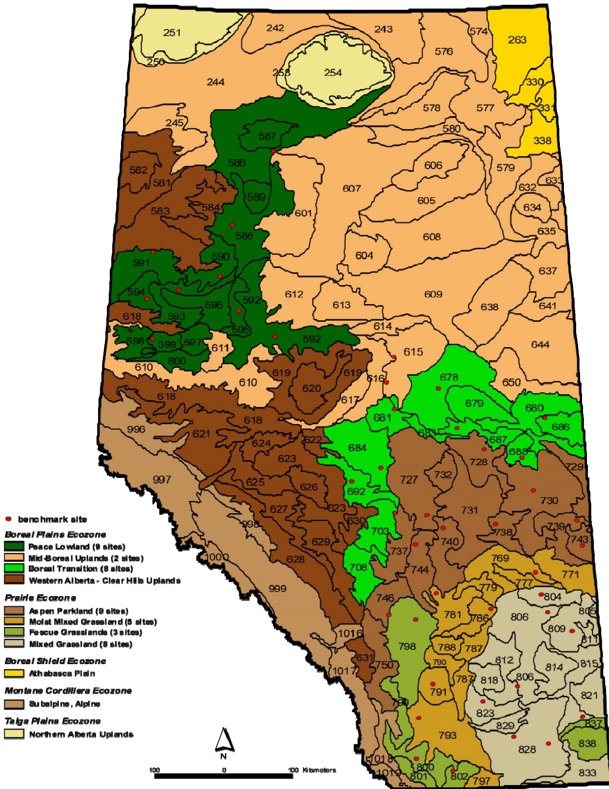
Location of the AESA Soil Quality Benchmark Sites
