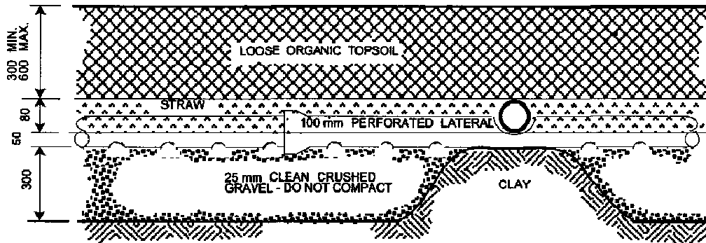
CROSS - SECTION THRU HEADER
