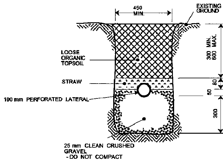
CROSS - SECTION THRU LATERAL TRENCH
