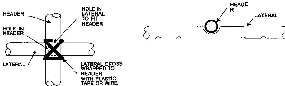
DETAILS OF LATERAL CROSSINGS
