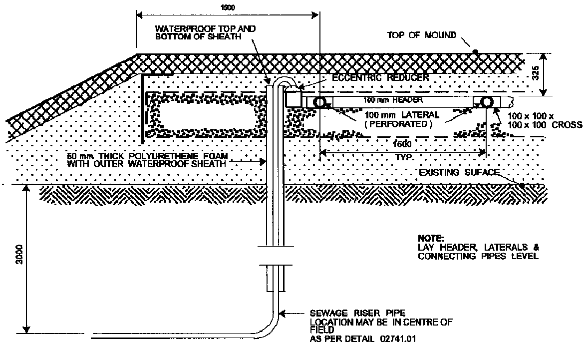
CROSS - SECTION THROUGH FIELD
