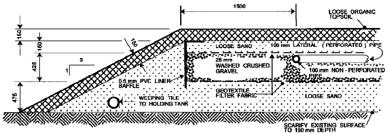
CROSS - SECTION THROUGH EDGE OF MOUND
