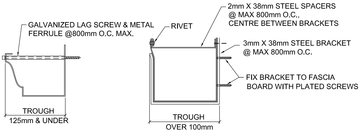
EAVE TROUGH DETAILS
